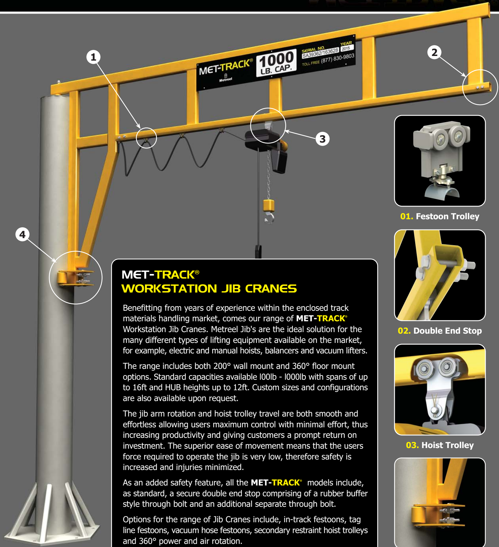
04. Roller Assembly
